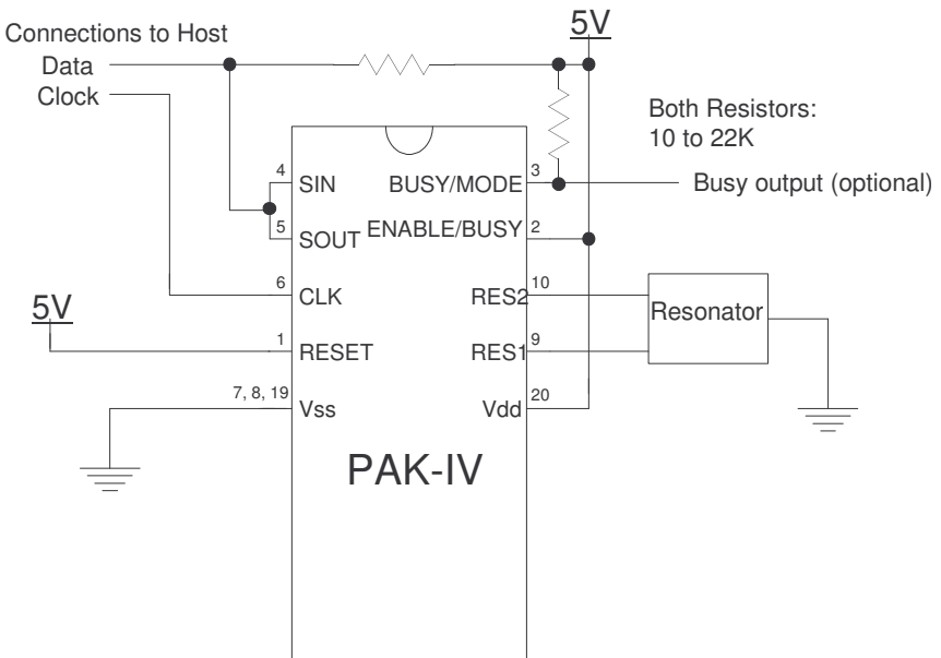
Example 1. Connections to Stamp or similar host
